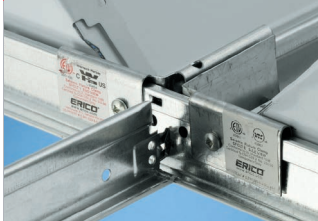
nVent CADDY Seismic Lighting Fixture Clamps SFCLT (consult catalog for all options)
