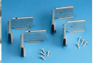
nVent CADDY Seismic Lighting Fixture Clamps SFCLT (consult catalog for all options)
